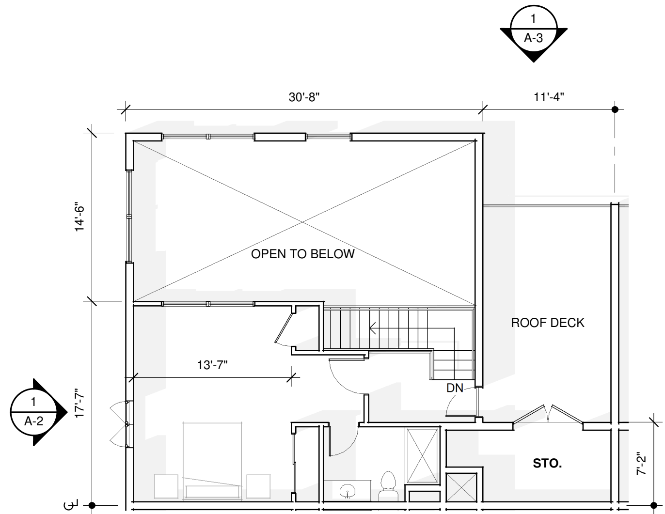
2 2nd Level - Typical Unit 1/8" = 1'-0"
