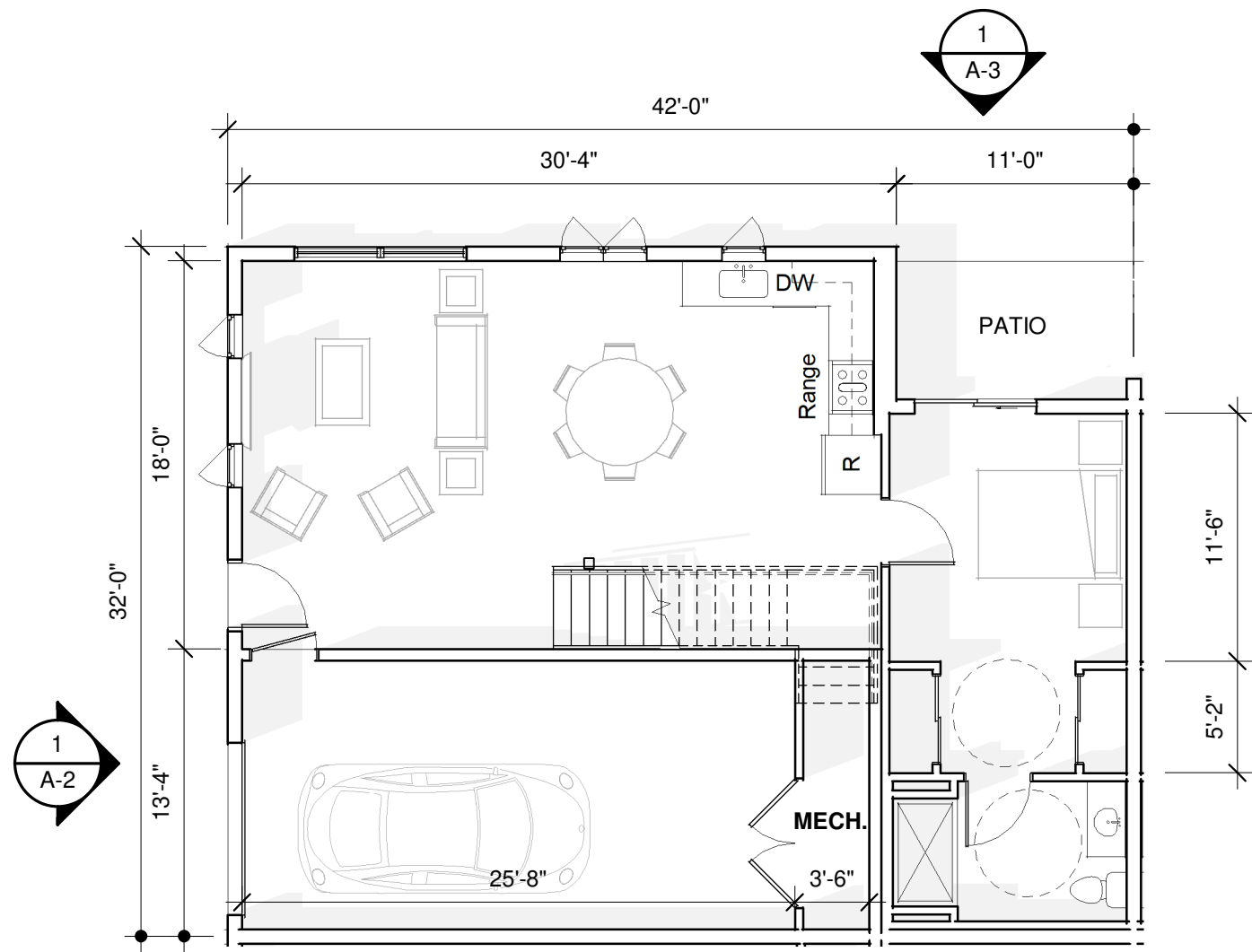
1 1st Floor - Typical Unit 1/8" = 1'-0"
